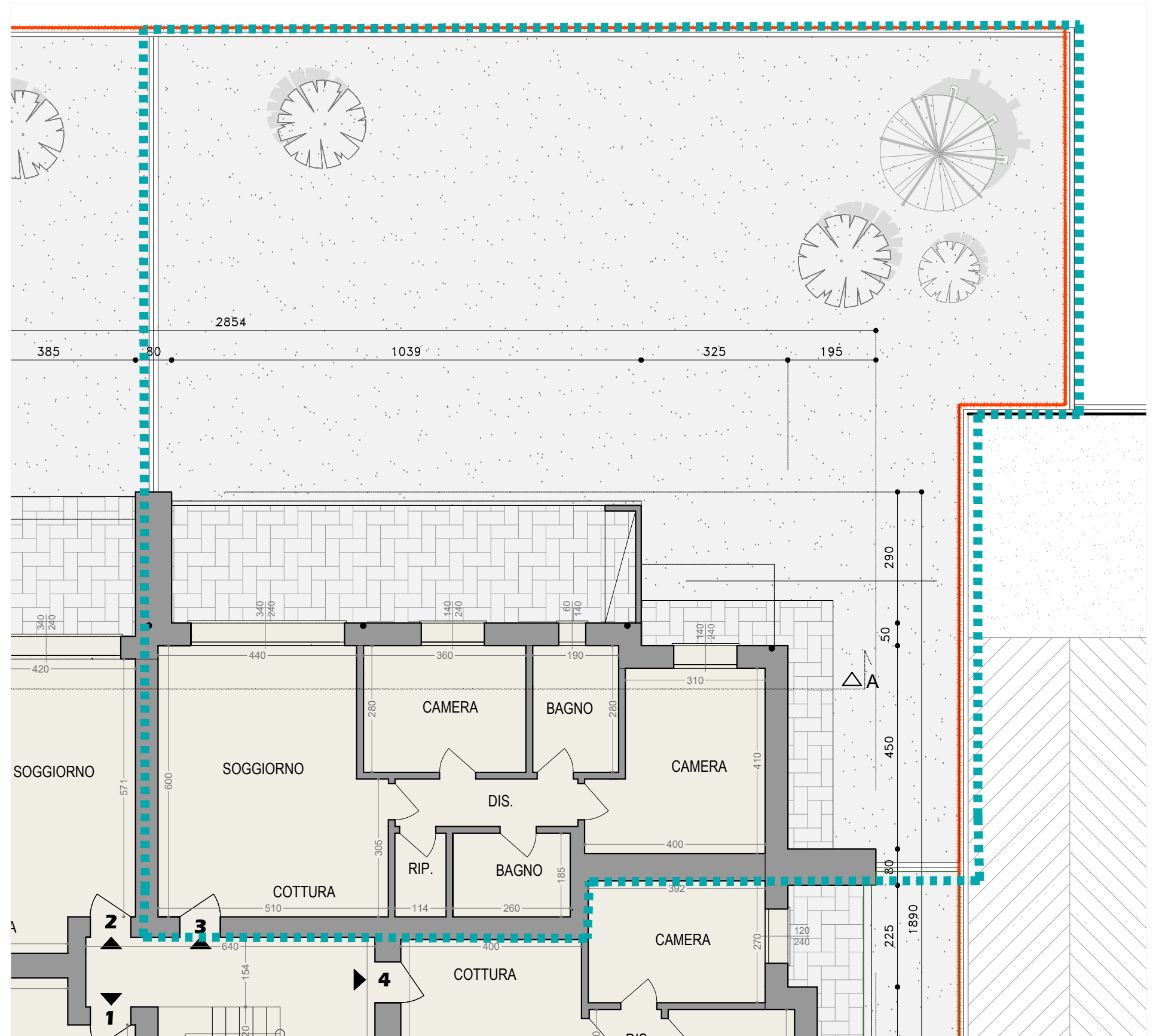
PIANO TERRA
